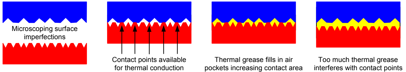
Figure 8: Micro-scoping surface interface
