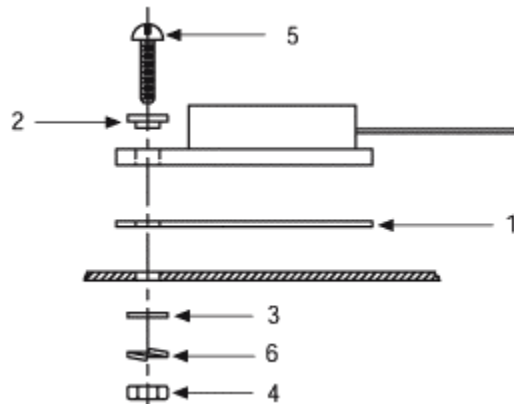
Figure 9: Mounting a device with a tab to a heatsink [5]
