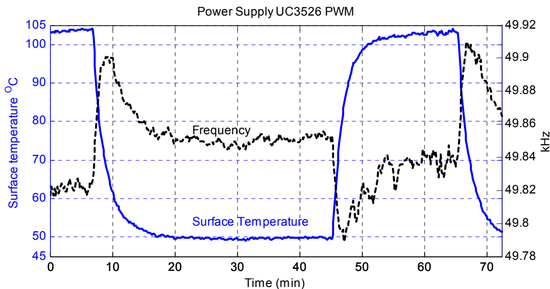
Figure 2: Oscillator frequency as a function of temperature
