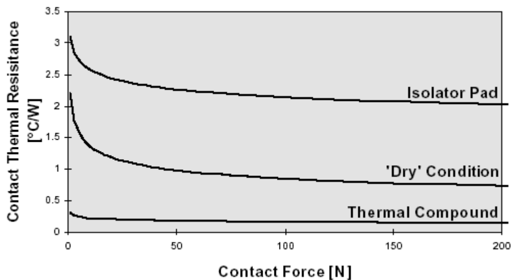
Figure 10: Thermal resistance vs. Contact force SUPER-247 [3]
