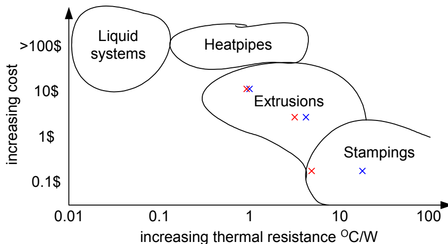
Figure 4: Cost vs. thermal resistance map
