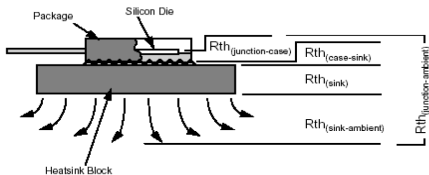
Figure 3: Thermal resistances in a system [3]
